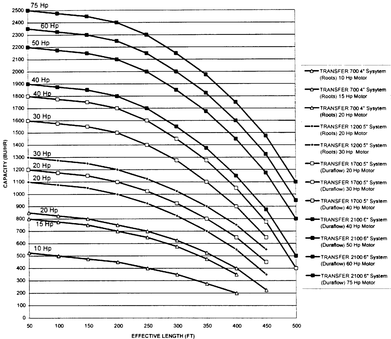
CAPACITY CHART 4", 5", & 6" SYSTEMS
